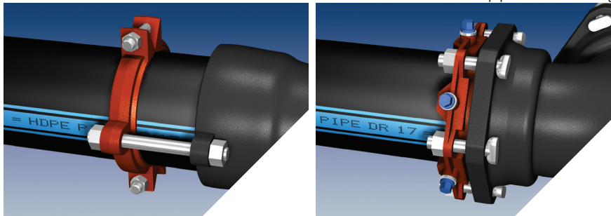
▲ Series 15PF06 on HDPE pipe at a push-on fitting.
