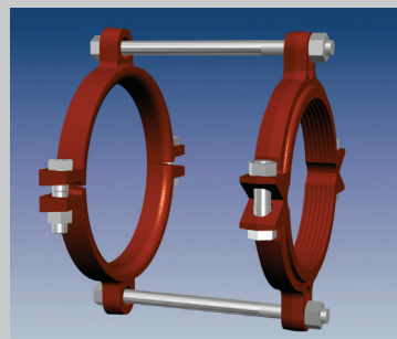
Sizes 4 - 8 inch
